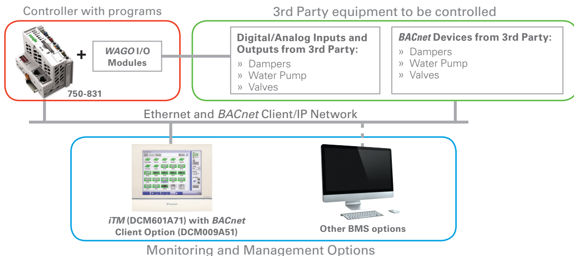
750-831 Daikin WAGO BACnet/IP Controller
