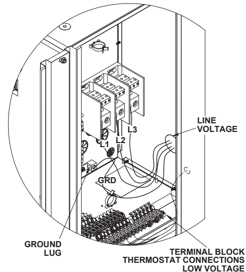
Thermostat Control Box
