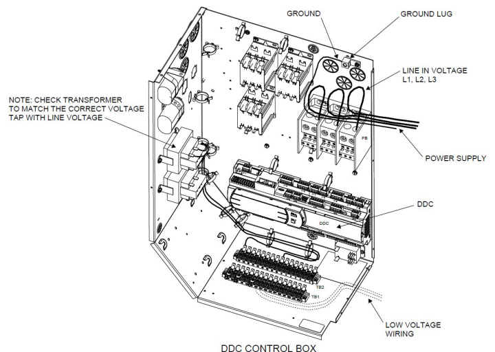
DDC Control Box
