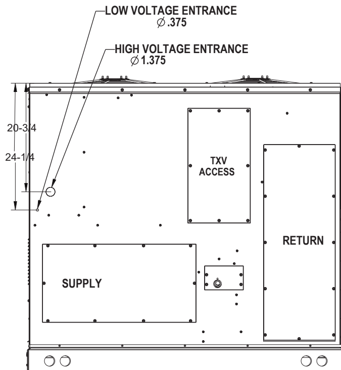
Thermostat Duct Panel
