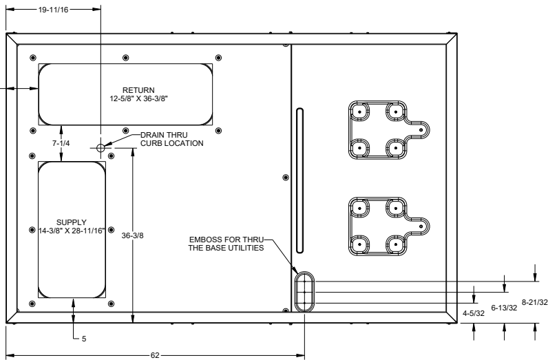
Vertical Discharge BOTTOM VIEW OF UNIT
