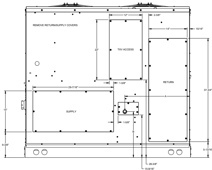
Horizontal Discharge Duct Connections|
