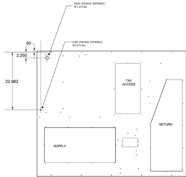
DDC Duct Panel
